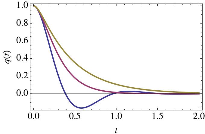
Figure 1: Overdamped (olive), critically damped (purple), and underdamped (blue) harmonic oscillators released from rest.
