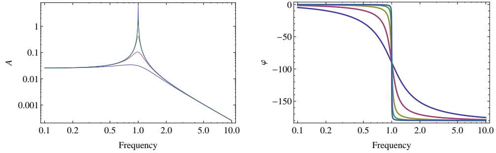
Figure 2: Amplitude and phase of a damped driven simple harmonic oscillator for several different quality factors ( Q = 1, 4, 16, 64 , and 256 ).
